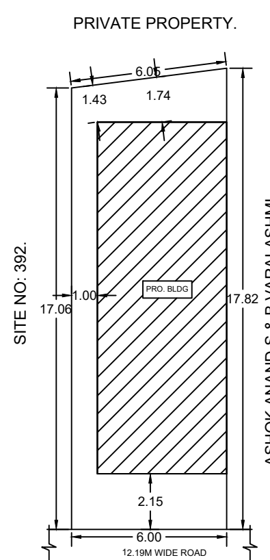
SITE PLAN
